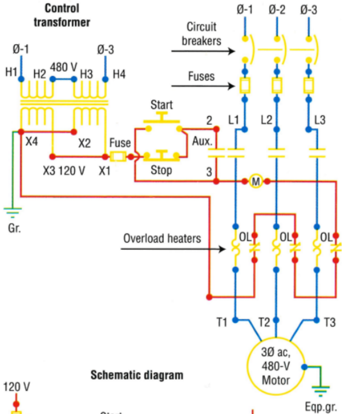
Wiring diagram
