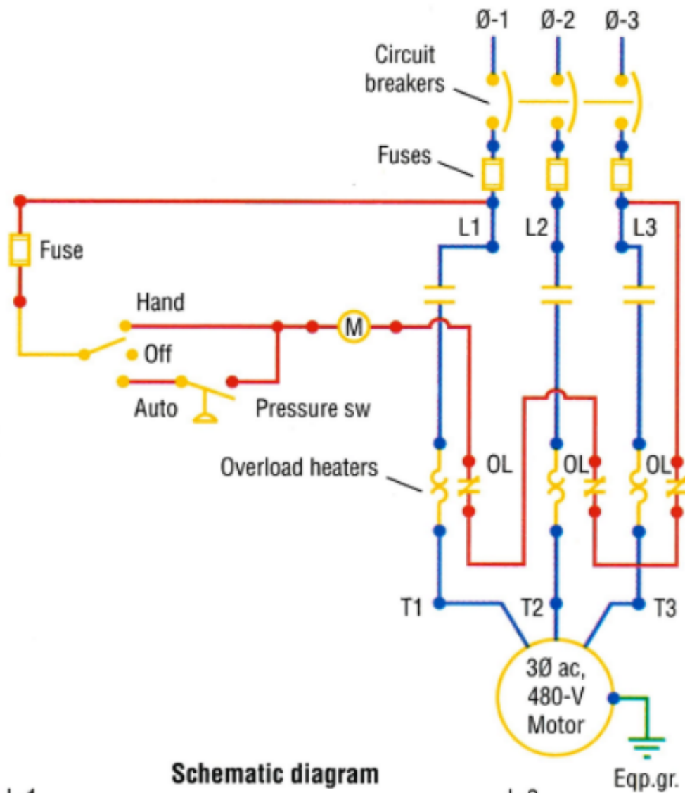
Wiring diagram
