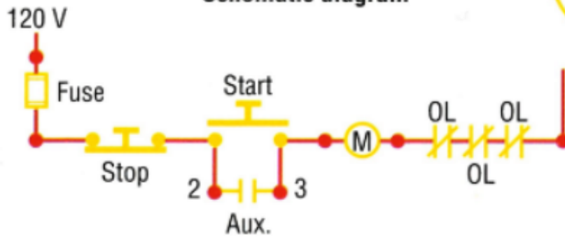
Schematic diagram
