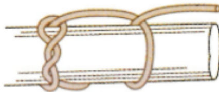
Timber hitch with half hitch
